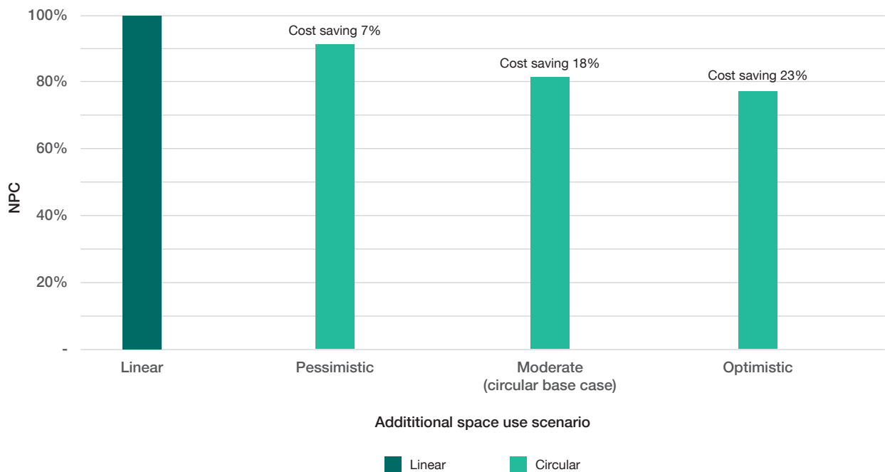
Figure 9. Sensitivity of NPC to different space use scenarios
